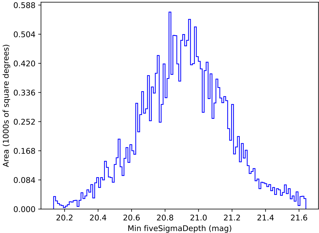
early_u_fpextra2.0_v3.4_10yrs All sky y band: Min fiveSigmaDepth
