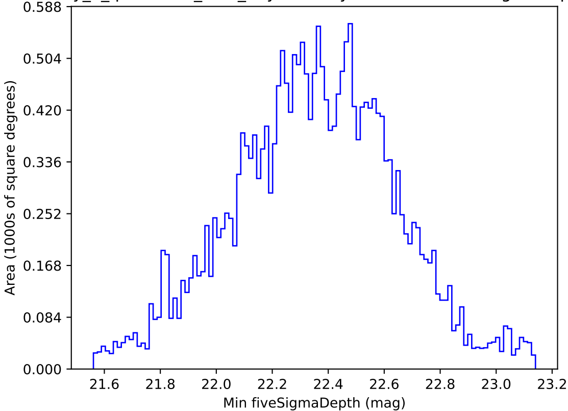
early_u_fpxtra2.0_v3.4_10yrs All sky u band: Min fiveSigmaDepth
