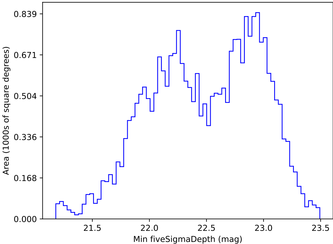
early_u_fpextra2.0_v3.4_10yrs All sky r band: Min fiveSigmaDepth
