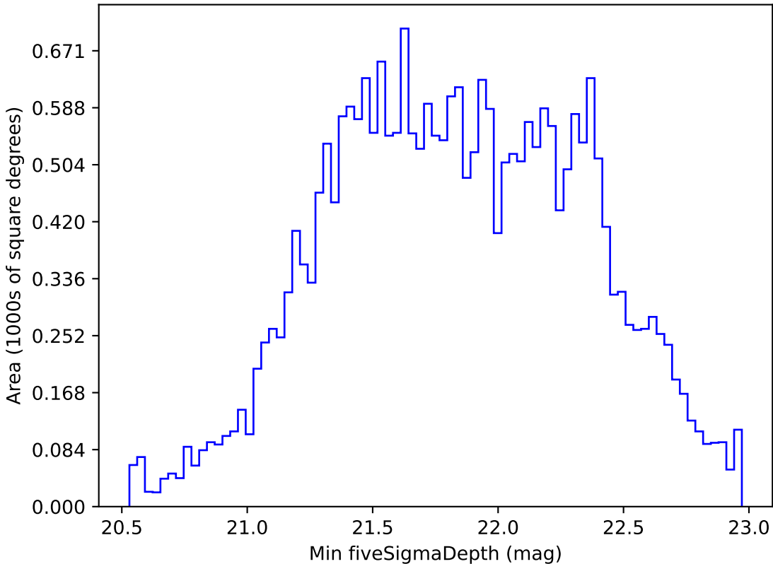
early_u_fpextra2.0_v3.4_10yrs All sky i band: Min fiveSigmaDepth
