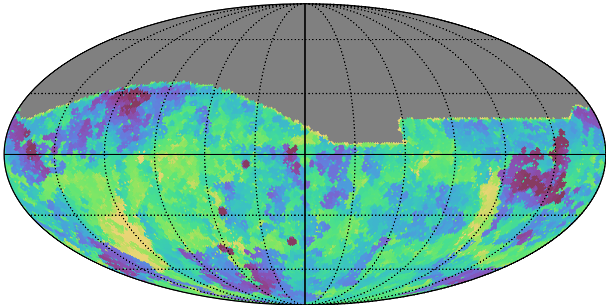
early_u_fpextra2.0_v3.4_10yrs All sky g band: Min fiveSigmaDepth
