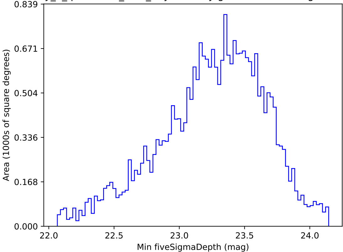
early_u_fpextra2.0_v3.4_10yrs All sky g band: Min fiveSigmaDepth
