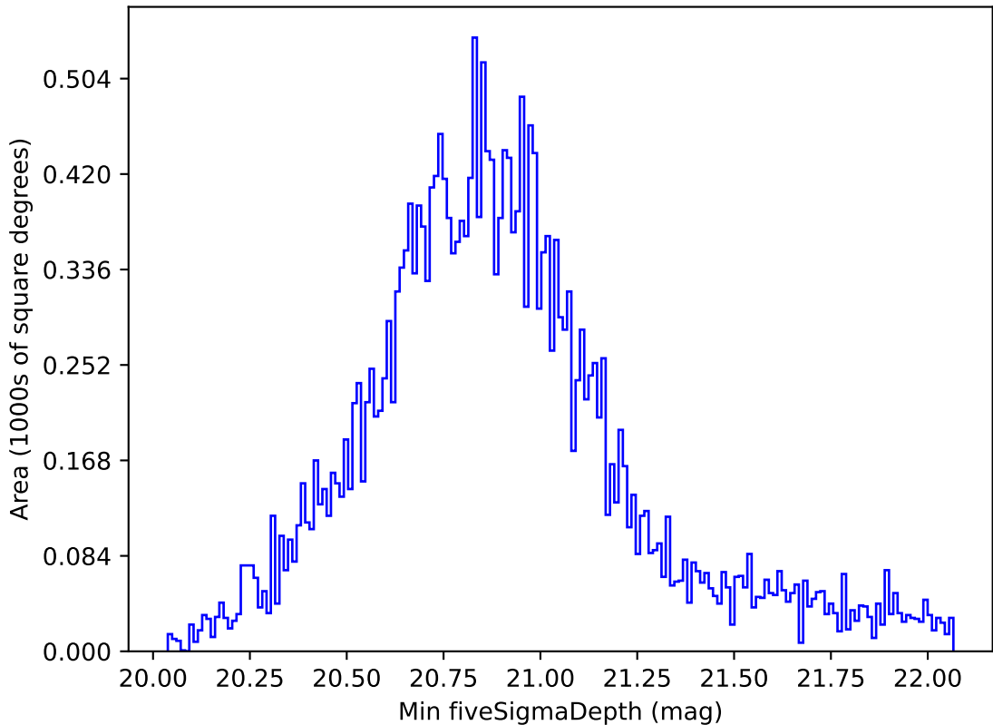
early_u_fpextra2.0_v3.4_10yrs All sky all bands: Min fiveSigmaDepth
