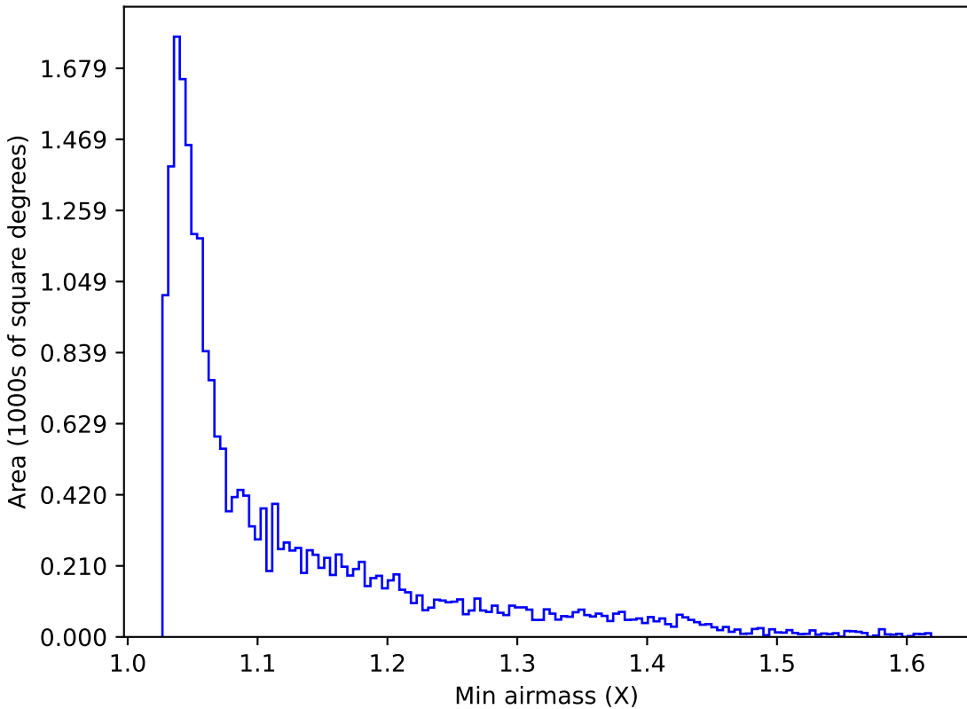
early_u_fpextra2.0_v3.4_10yrs Yr 1 y band: Min airmass
