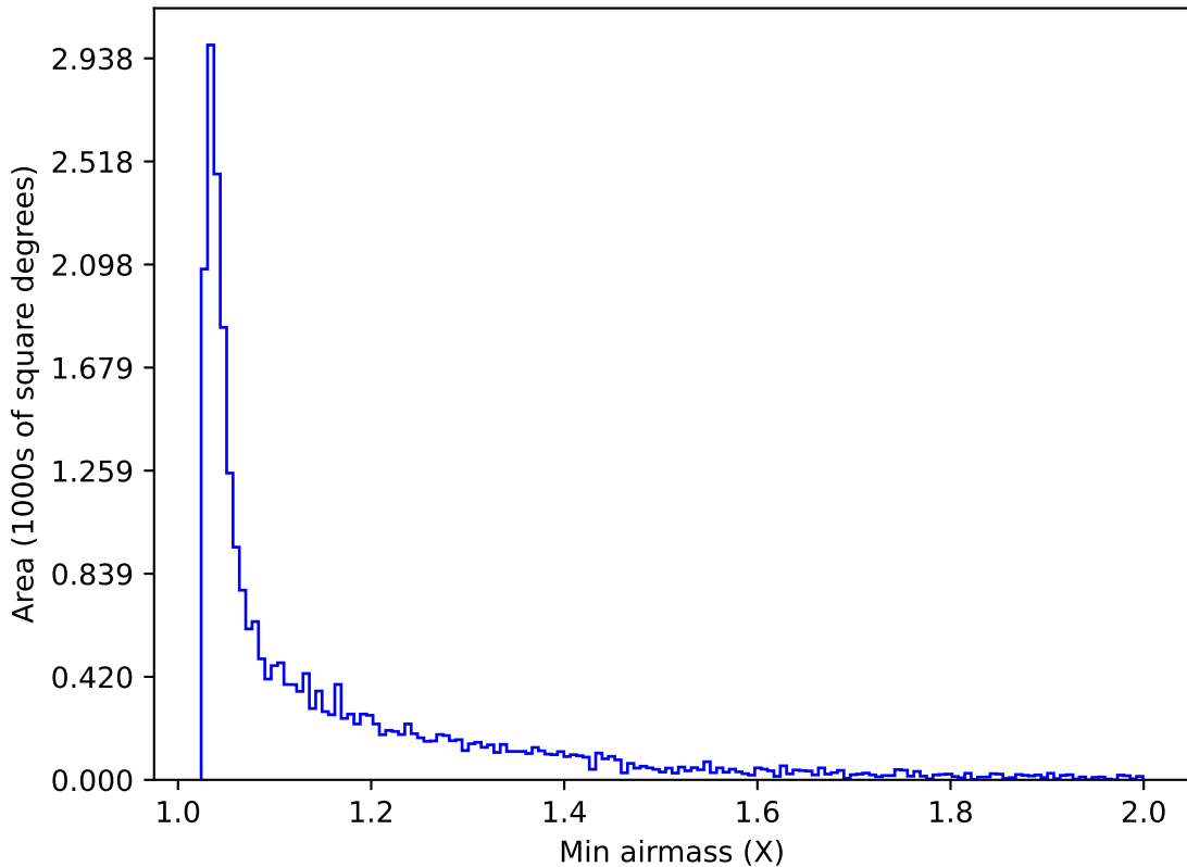
early_u_fpextra2.0_v3.4_10yrs Yr 1 i band: Min airmass
