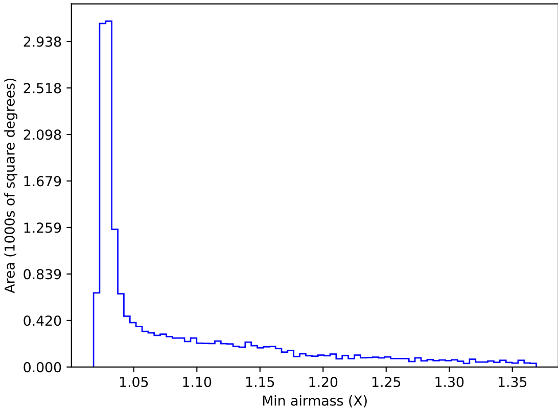
early_u_fpextra2.0_v3.4_10yrs WFD z band: Min airmass
