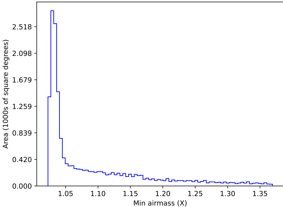
early_u_fpextra2.0_v3.4_10yrs WFD y band: Min airmass
