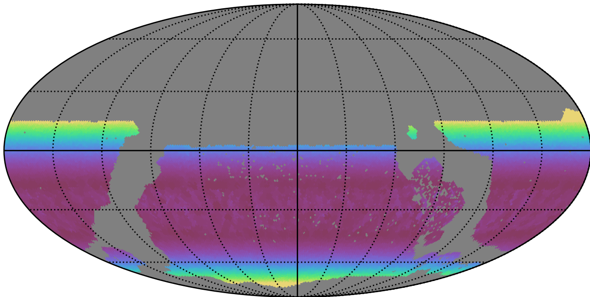
early_u_fpextra2.0_v3.4_10yrs WFD u band: Min airmass
