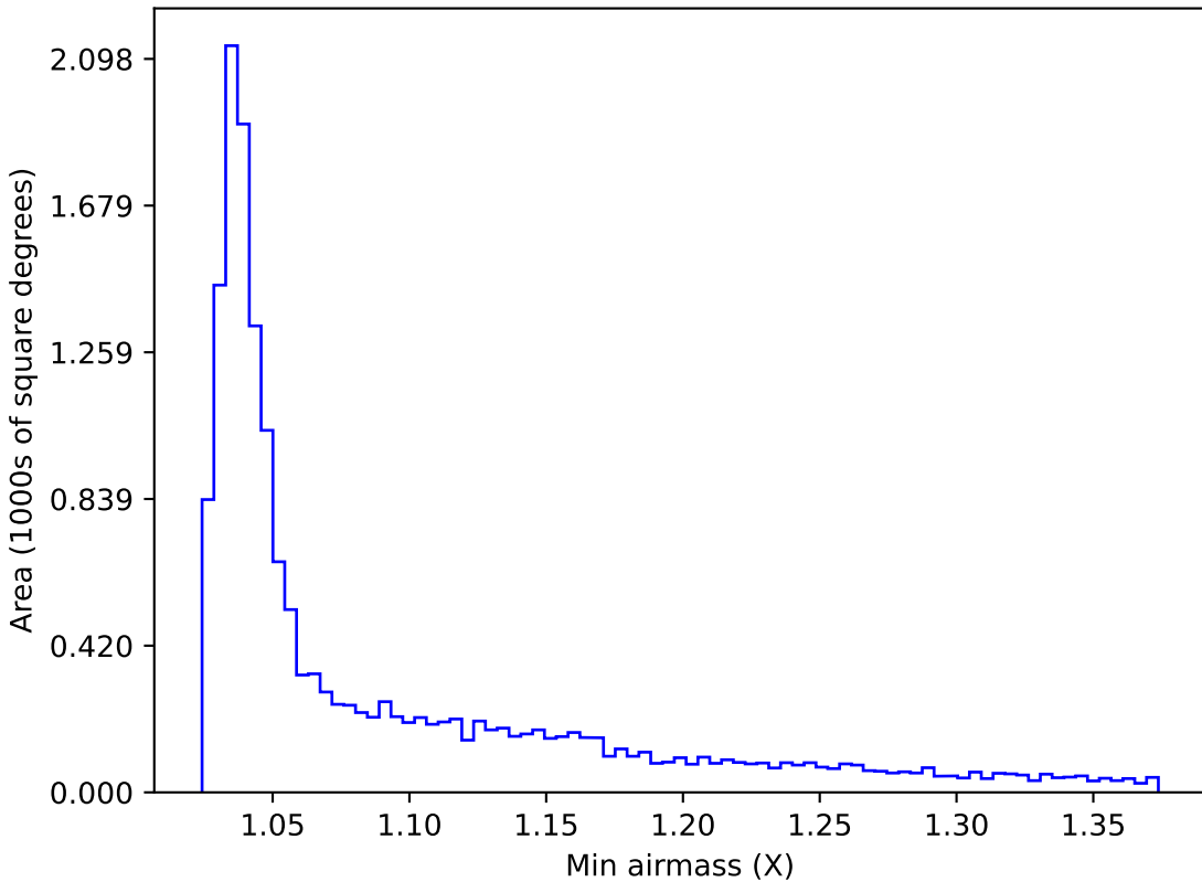
early_u_fpextra2.0_v3.4_10yrs WFD u band: Min airmass
