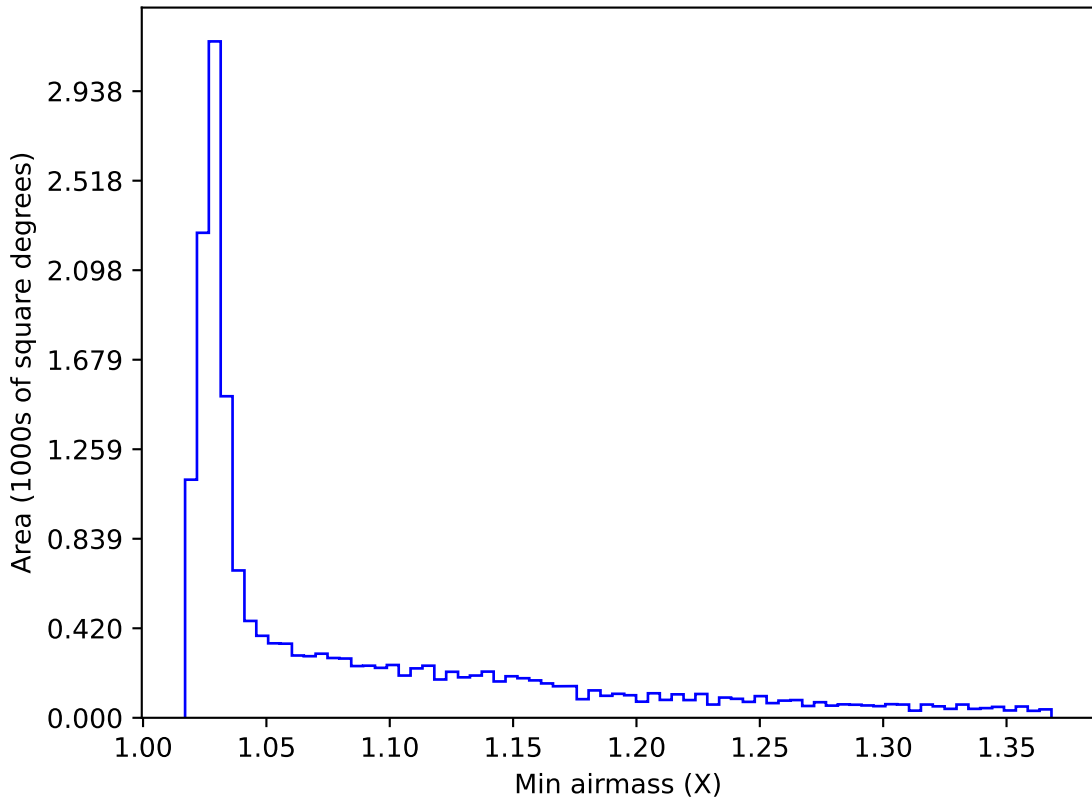
early_u_fpextra2.0_v3.4_10yrs WFD r band: Min airmass
