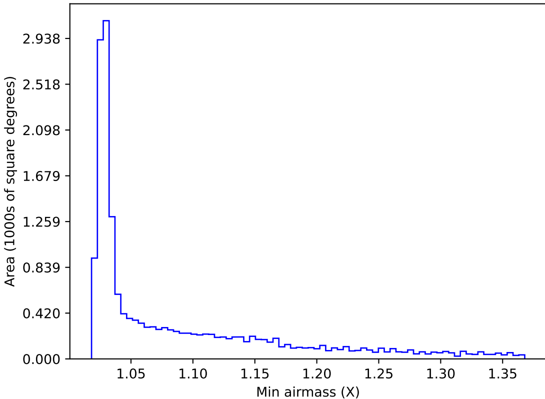
early_u_fpextra2.0_v3.4_10yrs WFD i band: Min airmass
