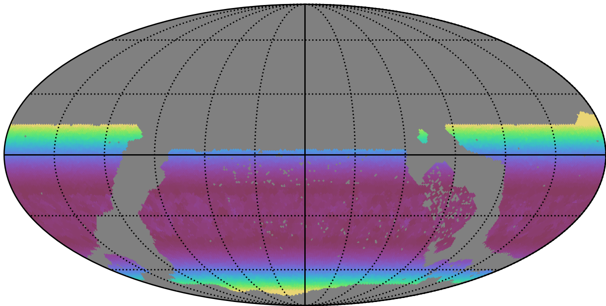
early_u_fpextra2.0_v3.4_10yrs WFD g band: Min airmass
