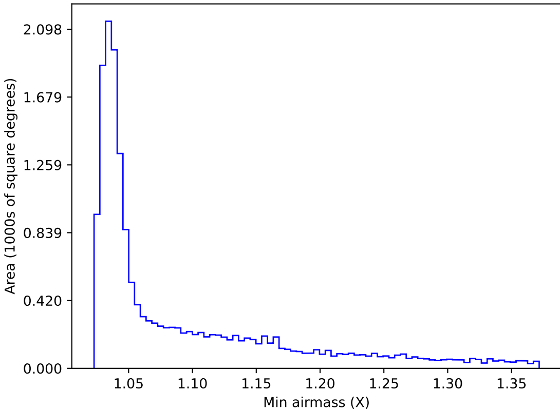
early_u_fpextra2.0_v3.4_10yrs WFD g band: Min airmass
