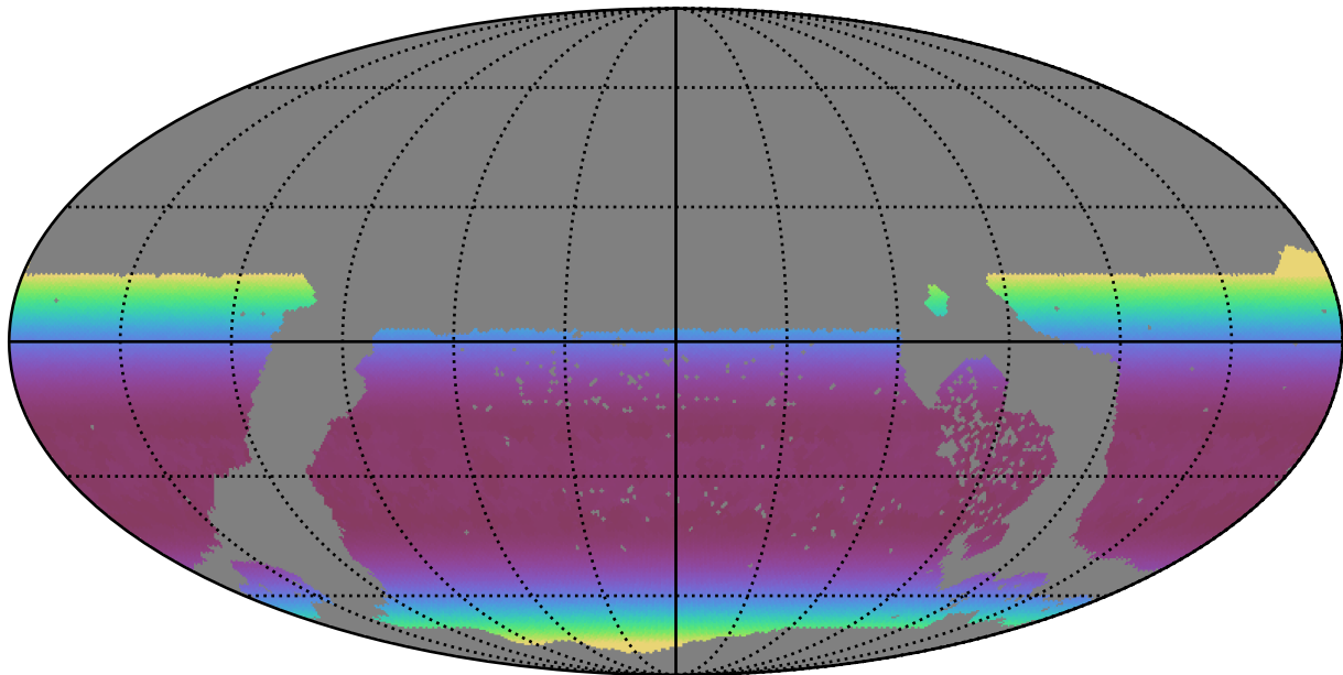
early_u_fpextra2.0_v3.4_10yrs WFD all bands: Min airmass
