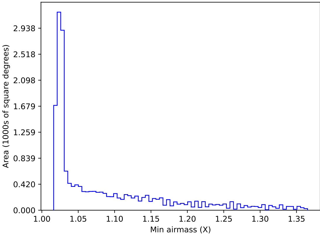
early_u_fpextra2.0_v3.4_10yrs WFD all bands: Min airmass
