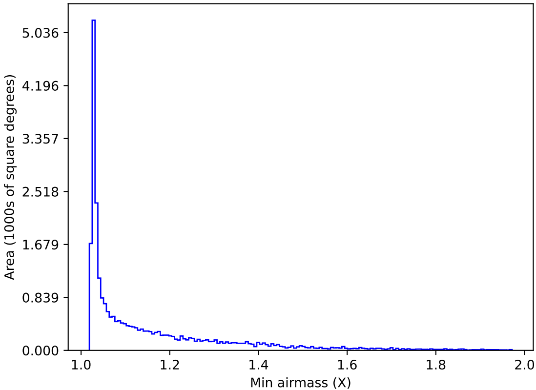
early_u_fpextra2.0_v3.4_10yrs All sky z band: Min airmass
