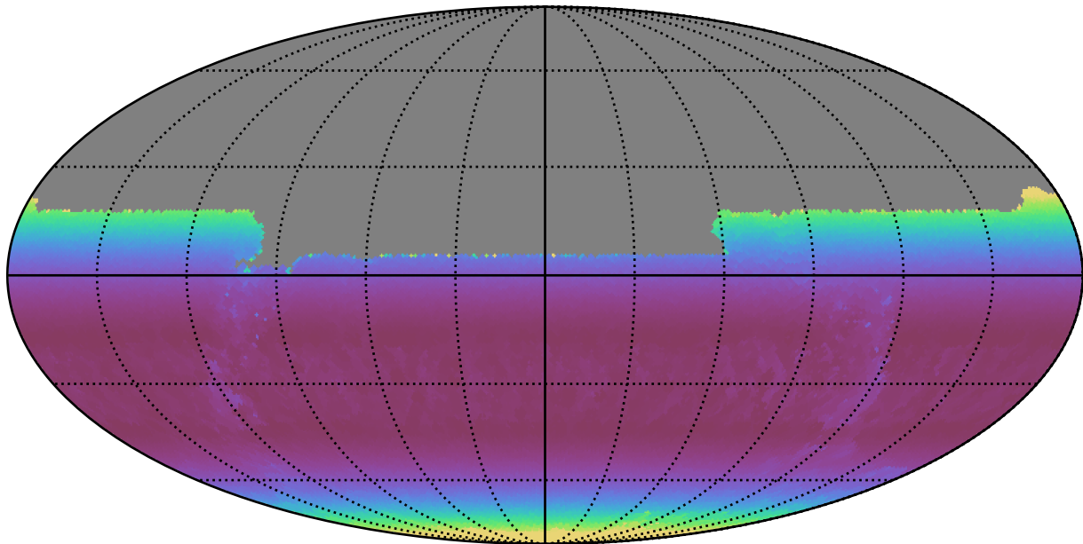
early_u_fpextra2.0_v3.4_10yrs All sky u band: Min airmass
