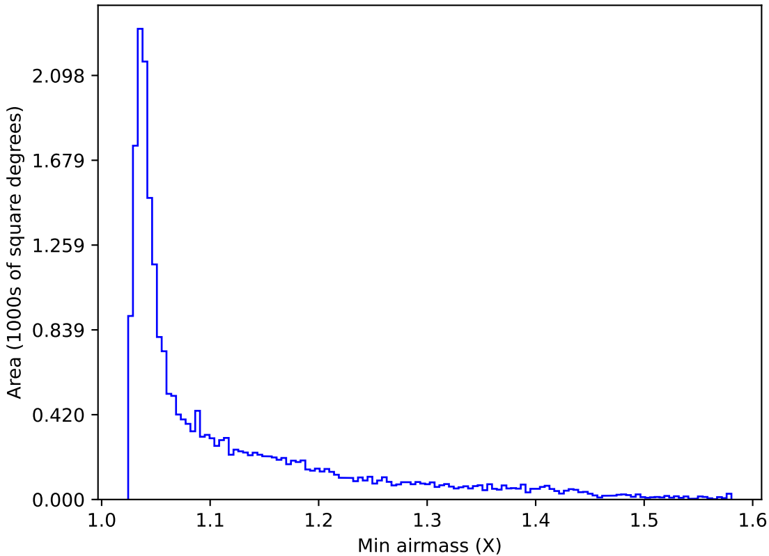
early_u_fpextra2.0_v3.4_10yrs All sky u band: Min airmass
