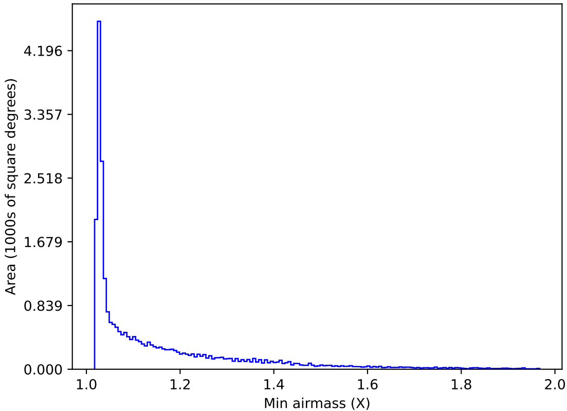
early_u_fpextra2.0_v3.4_10yrs All sky r band: Min airmass
