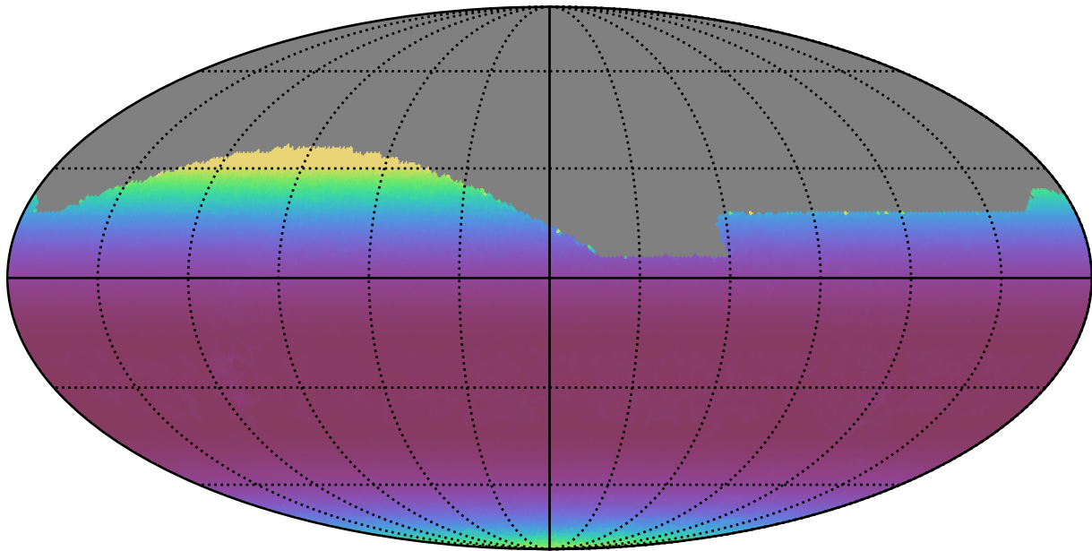
early_u_fpextra2.0_v3.4_10yrs All sky i band: Min airmass
