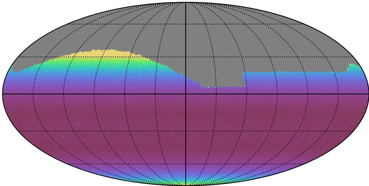
early_u_fpextra2.0_v3.4_10yrs All sky g band: Min airmass
