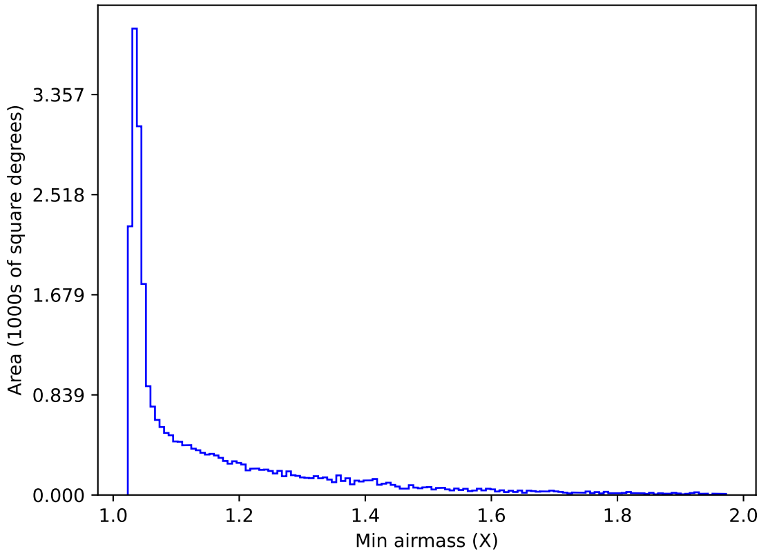
early_u_fpextra2.0_v3.4_10yrs All sky g band: Min airmass
