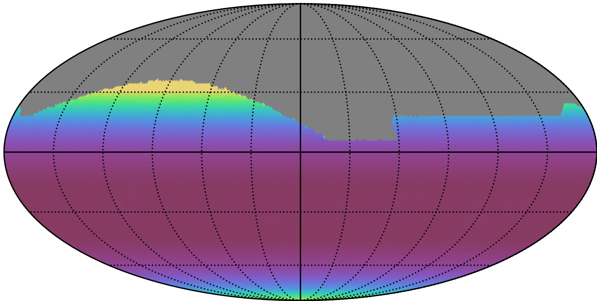
early_u_fpextra2.0_v3.4_10yrs All sky all bands: Min airmass
