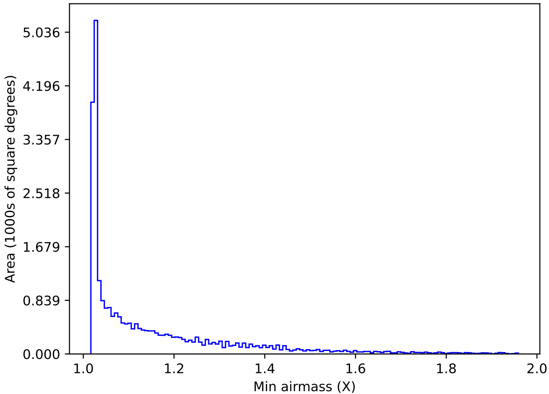
early_u_fpextra2.0_v3.4_10yrs All sky all bands: Min airmass
