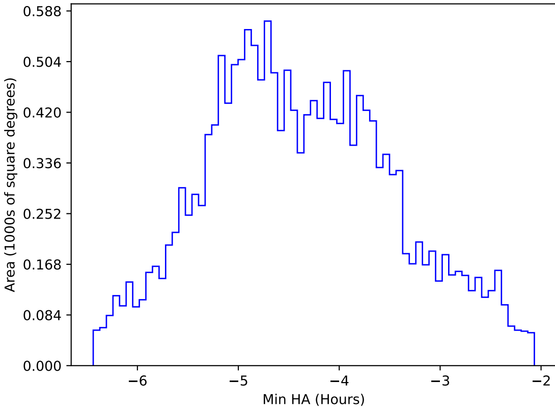
early_u_fpextra2.0_v3.4_10yrs WFD z band: Min HA
