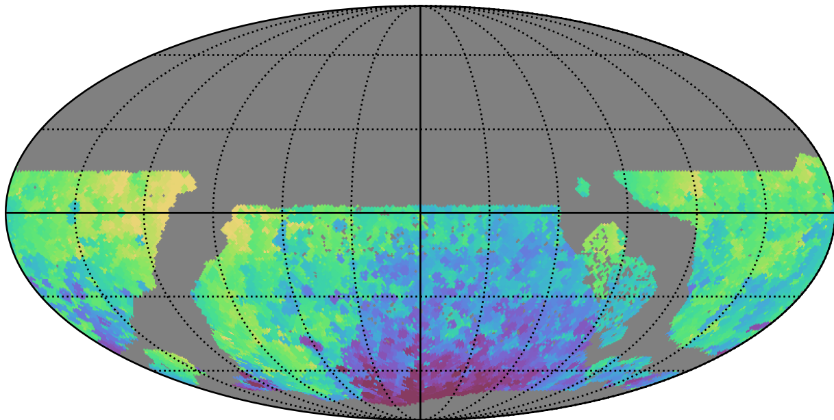
early_u_fpextra2.0_v3.4_10yrs WFD y band: Min HA
