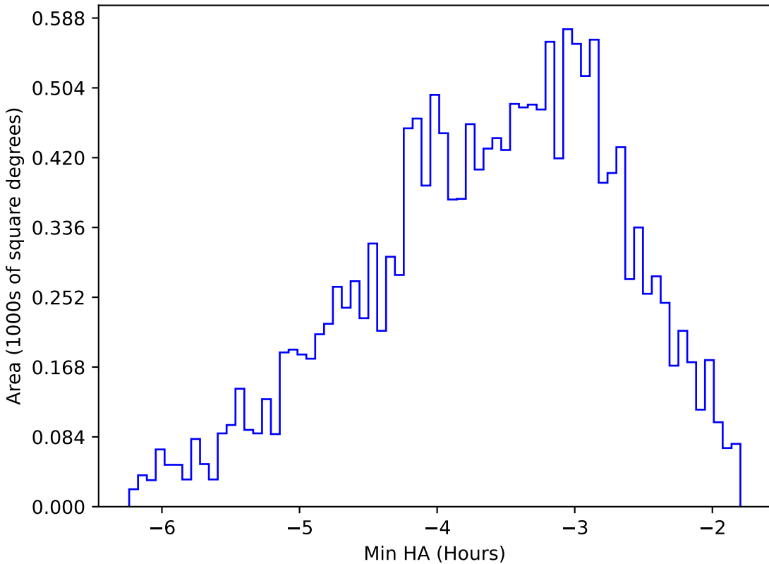
early_u_fpextra2.0_v3.4_10yrs WFD y band: Min HA
