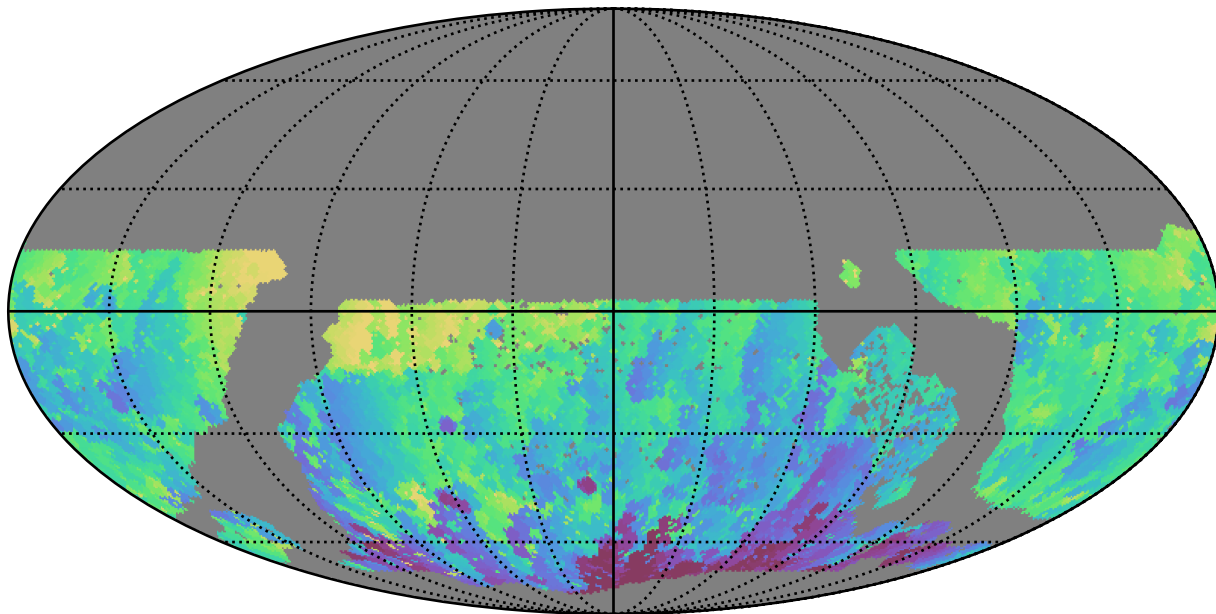
early_u_fpextra2.0_v3.4_10yrs WFD u band: Min HA
