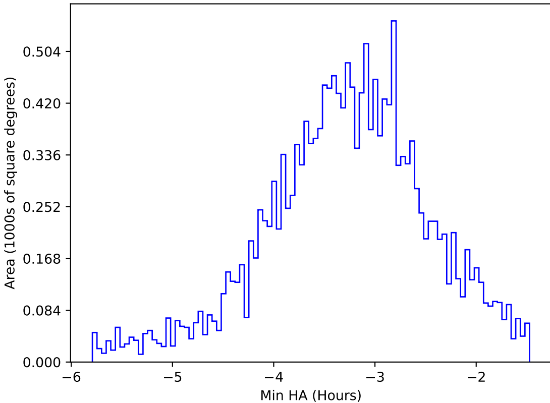
early_u_fpextra2.0_v3.4_10yrs WFD u band: Min HA
