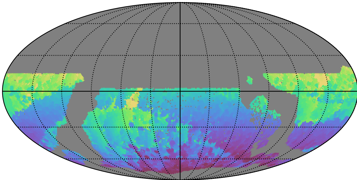
early_u_fpextra2.0_v3.4_10yrs WFD r band: Min HA
