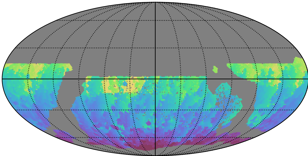
early_u_fpextra2.0_v3.4_10yrs WFD g band: Min HA
