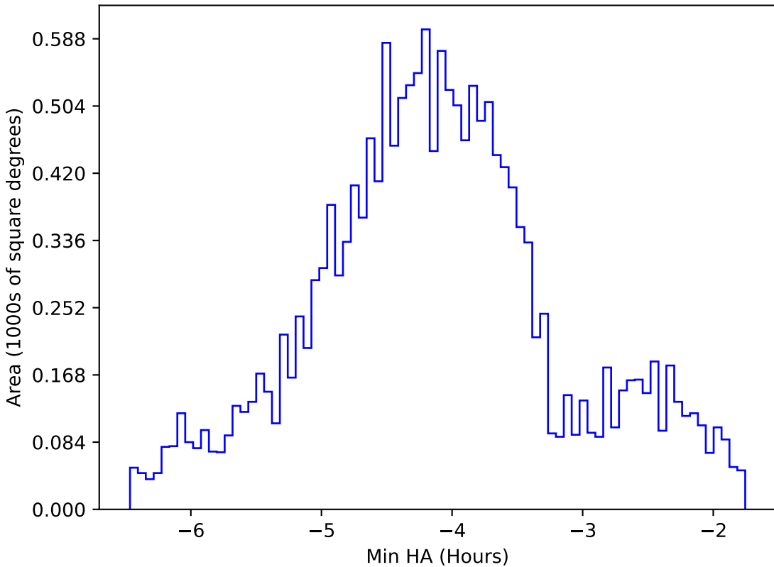
early_u_fpextra2.0_v3.4_10yrs WFD g band: Min HA
