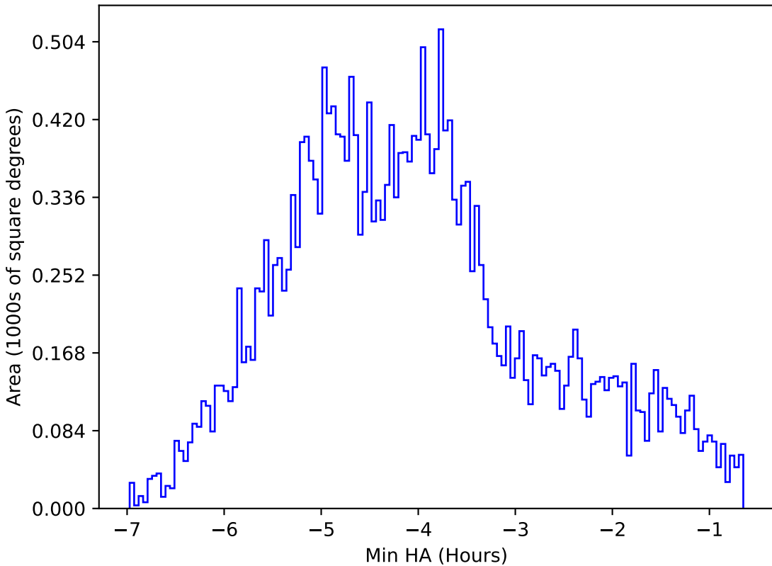
early_u_fpextra2.0_v3.4_10yrs All sky z band: Min HA
