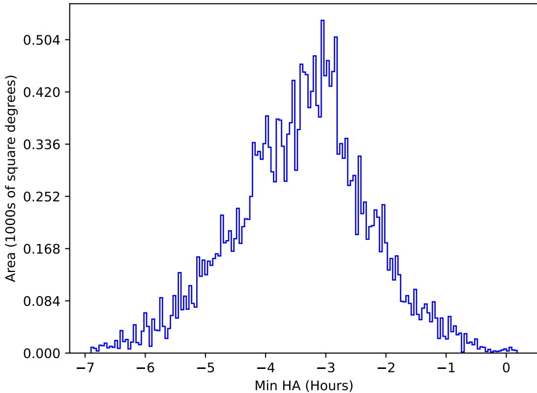
early_u_fpextra2.0_v3.4_10yrs All sky y band: Min HA
