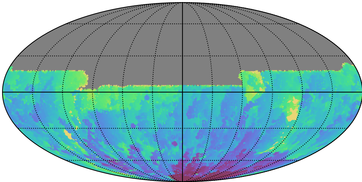
early_u_fpextra2.0_v3.4_10yrs All sky u band: Min HA
