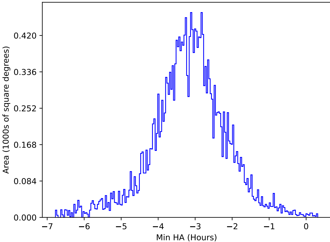
early_u_fpextra2.0_v3.4_10yrs All sky u band: Min HA
