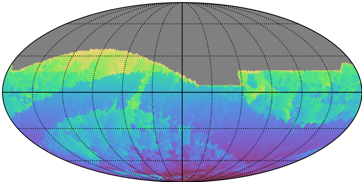
early_u_fpextra2.0_v3.4_10yrs All sky r band: Min HA
