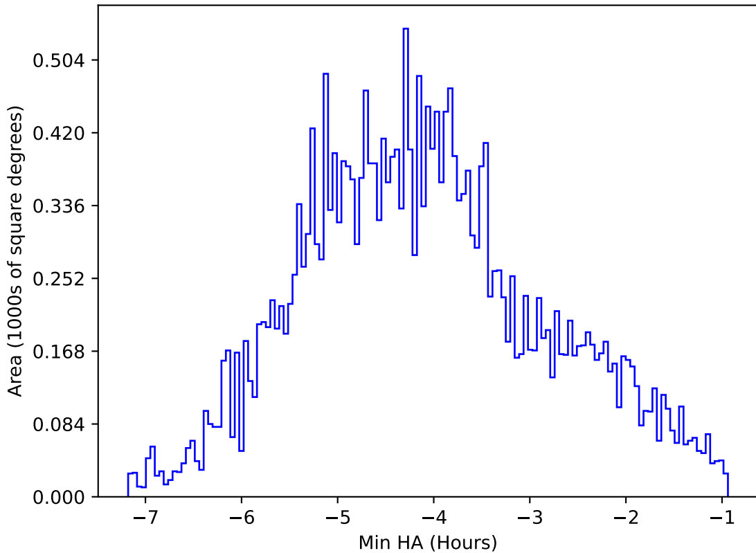
early_u_fpextra2.0_v3.4_10yrs All sky i band: Min HA
