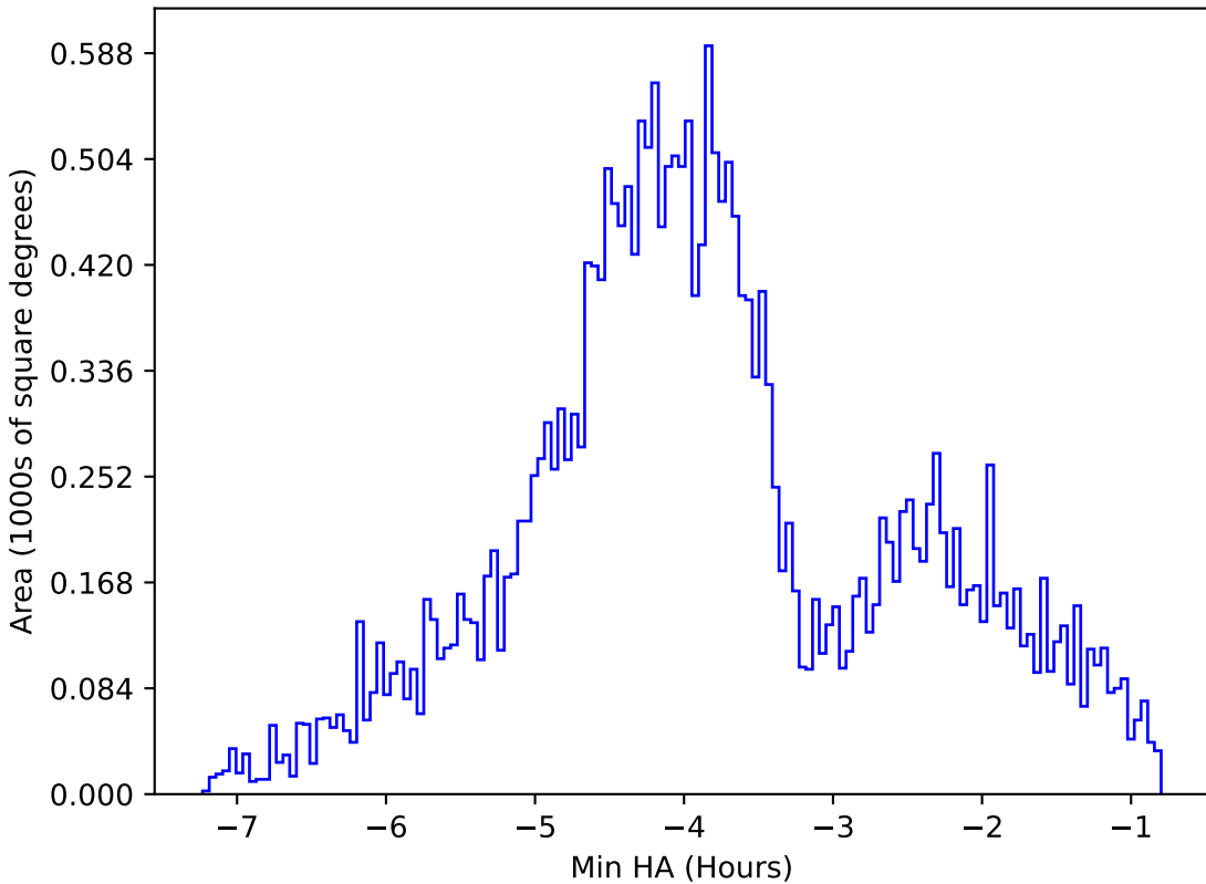
early_u_fpextra2.0_v3.4_10yrs All sky g band: Min HA
