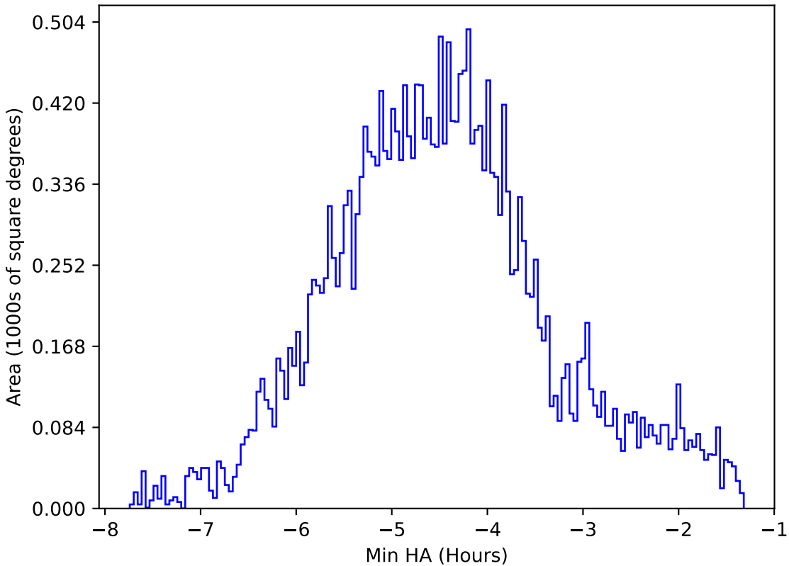
early_u_fpextra2.0_v3.4_10yrs All sky all bands: Min HA
