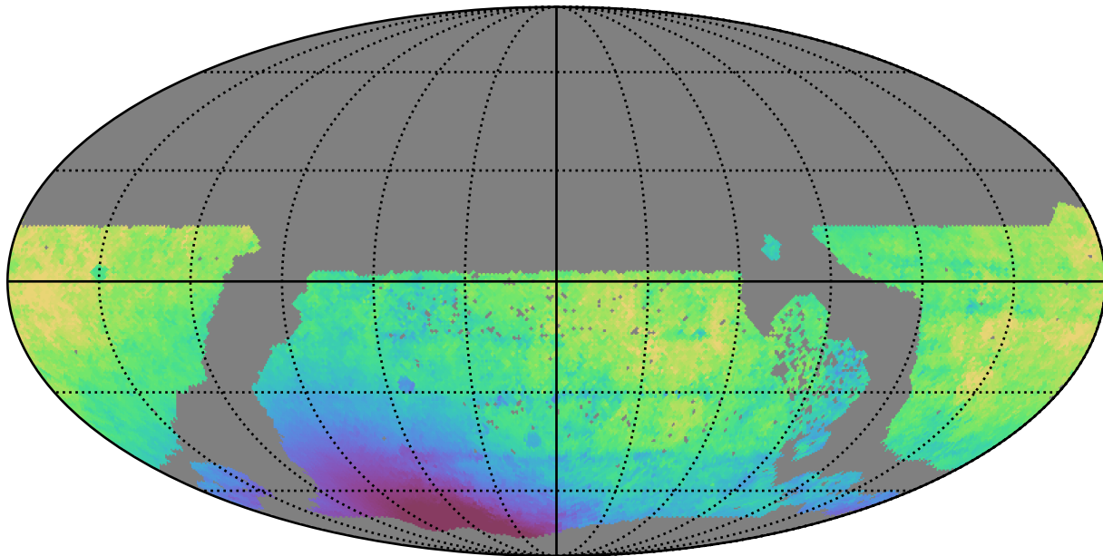
early_u_fpextra2.0_v3.4_10yrs WFD z band: Median solarElong
