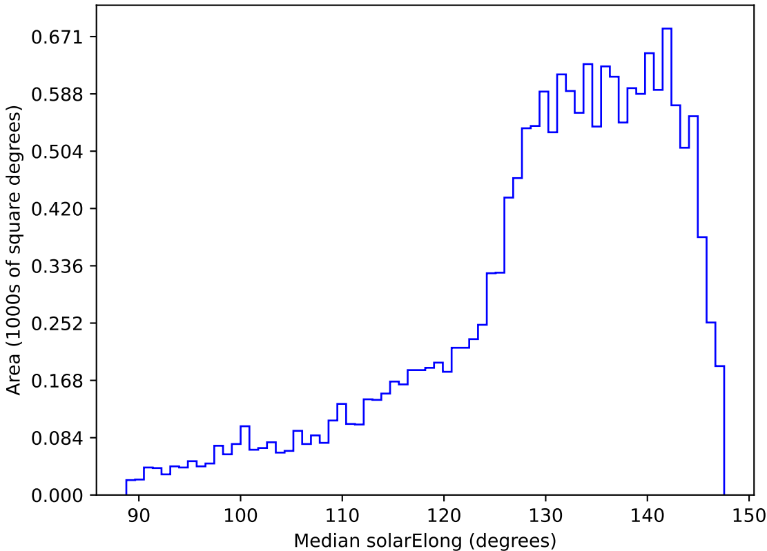
early_u_fpextra2.0_v3.4_10yrs WFD y band: Median solarElong
