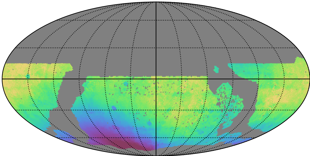
early_u_fpextra2.0_v3.4_10yrs WFD r band: Median solarElong
