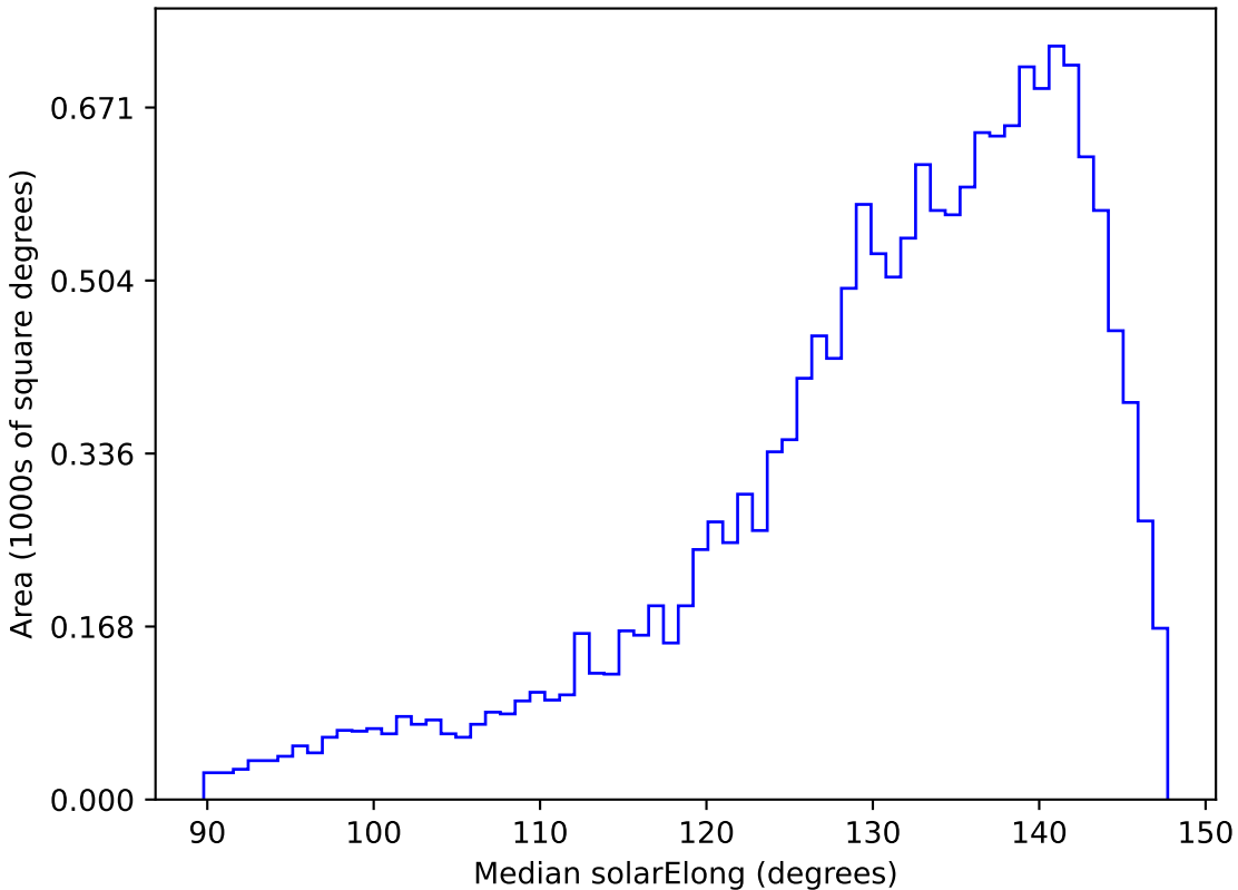
early_u_fpextra2.0_v3.4_10yrs WFD r band: Median solarElong
