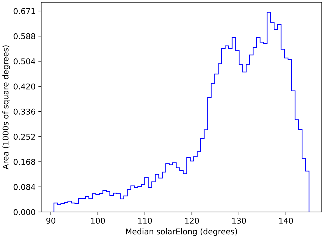
early_u_fpextra2.0_v3.4_10yrs WFD i band: Median solarElong
