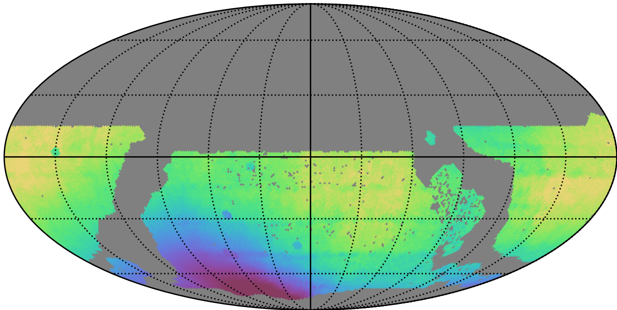
early_u_fpextra2.0_v3.4_10yrs WFD all bands: Median solarElong
